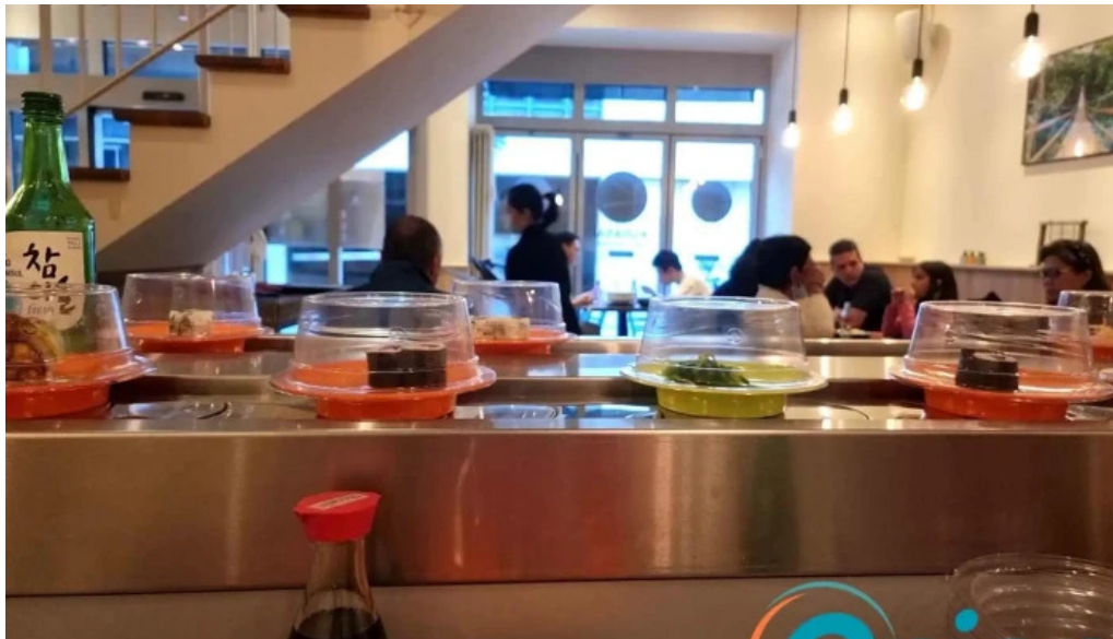
Kudasai atmosphere
